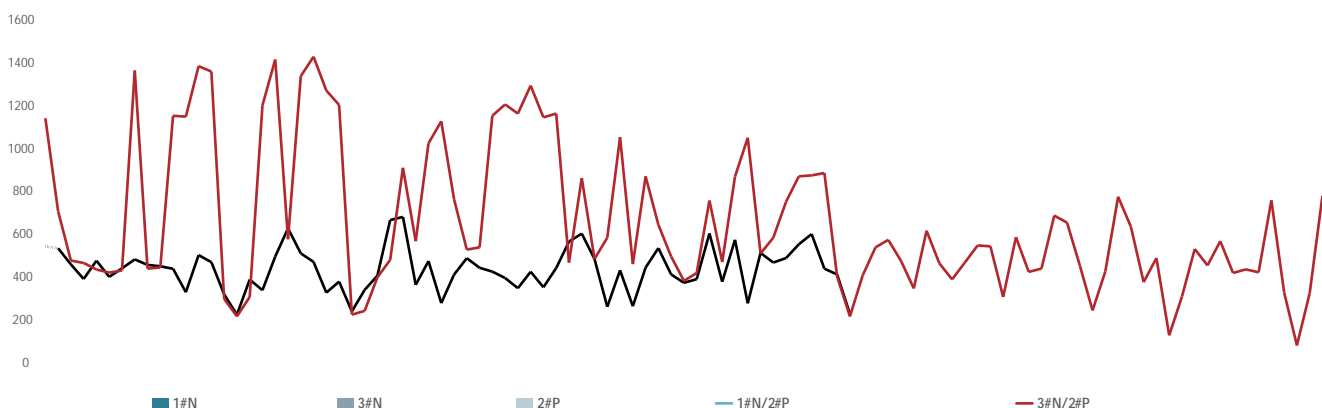
Figure 1: Comparison of daily energy yield of N-type and P-type modules
